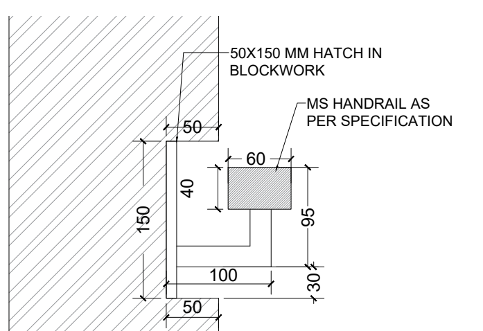
RAILING DETAIL
