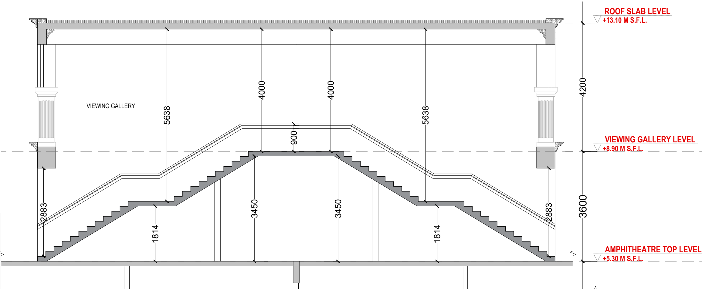
SECTION
