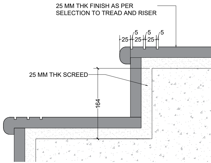
TYPICAL TREAD RISER DETAIL
