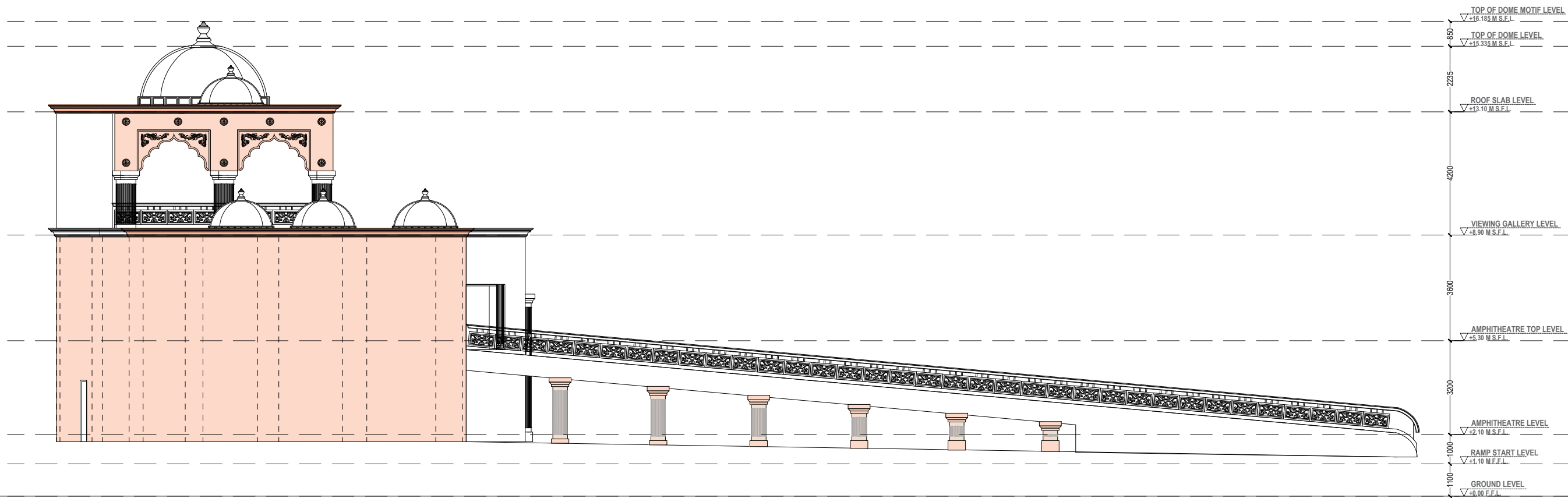
WEST ELEVATION
