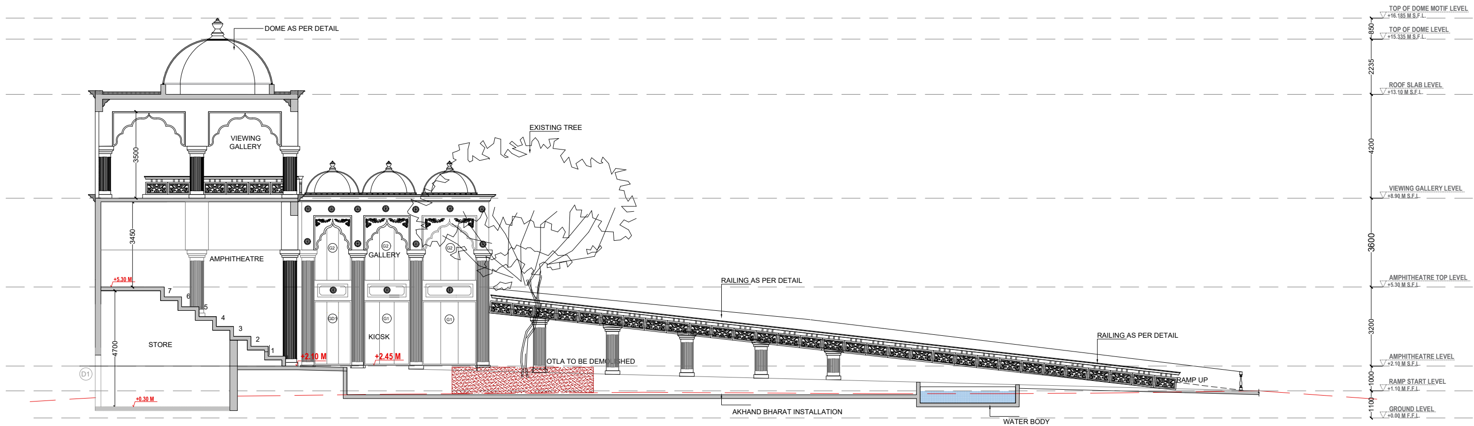
SECTION AA
